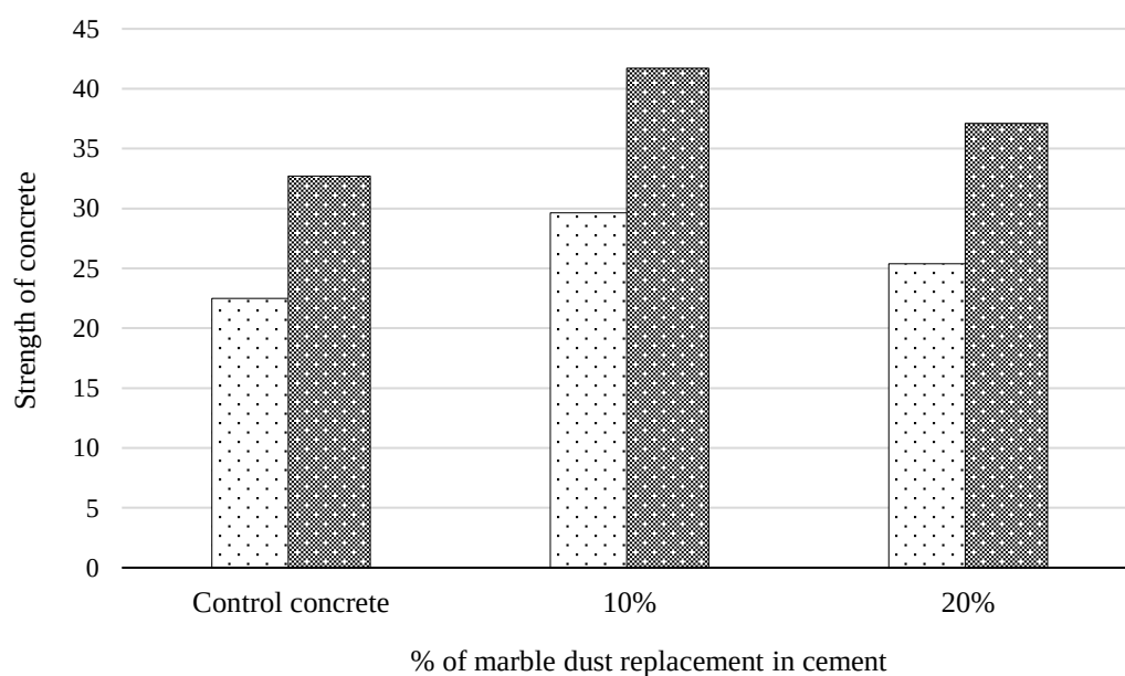
Figure 1. Compressive strength.
