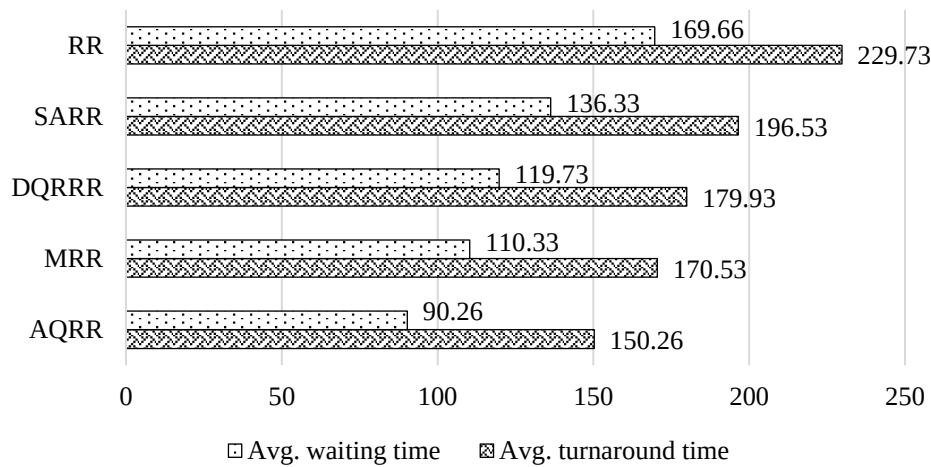
Figure 5. Comparative study of avg waiting time and avg turnaround time between RR, SARR algorithms.
