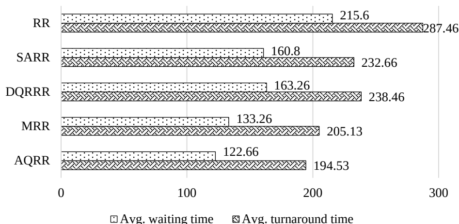
Figure 4. Comparative study of avg. waiting time and avg turnaround time among RR, SARR, DQRRR, MRR, and AQRR scheduling algorithms.
