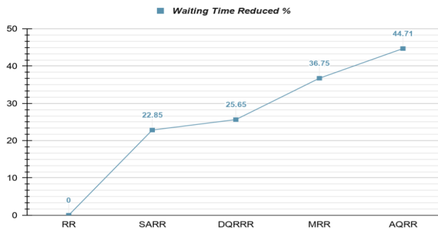
Figure 7. Percentage of waiting time reduced.
