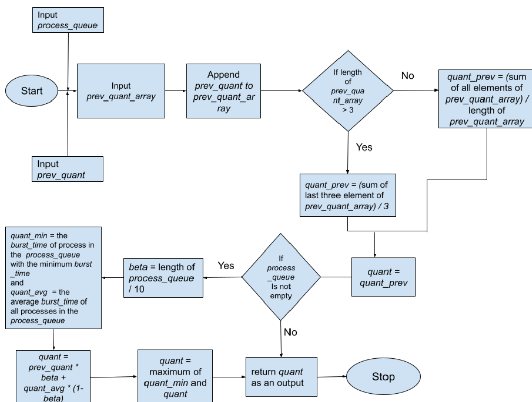
Figure 3. (b) Flowchart of quantum update: Case 2.
