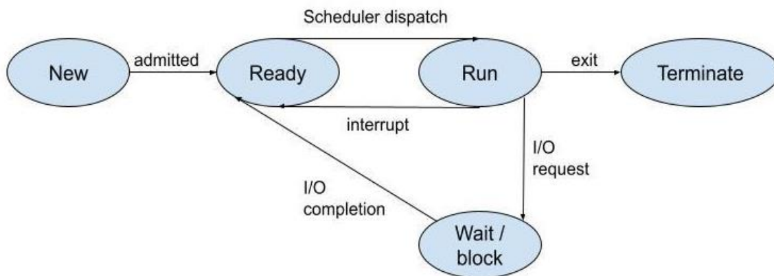
Figure 1. Stages of processes in CPU scheduling.
