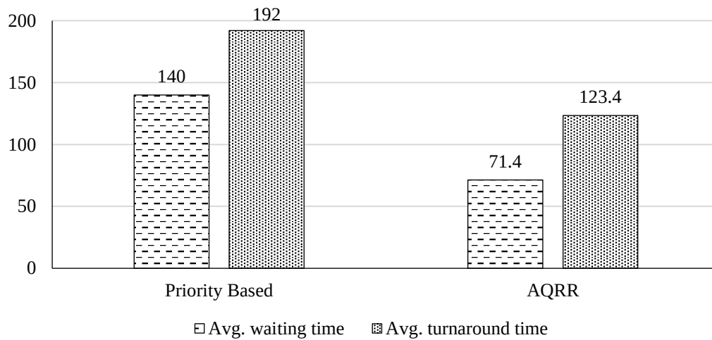
Figure 6. Graphical representation of comparison between preemptive priority based and AQRR scheduling.
