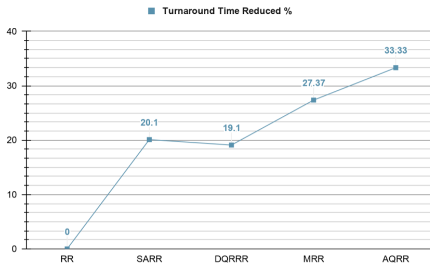
Figure 8. Percentage of turnaround time reduced.
