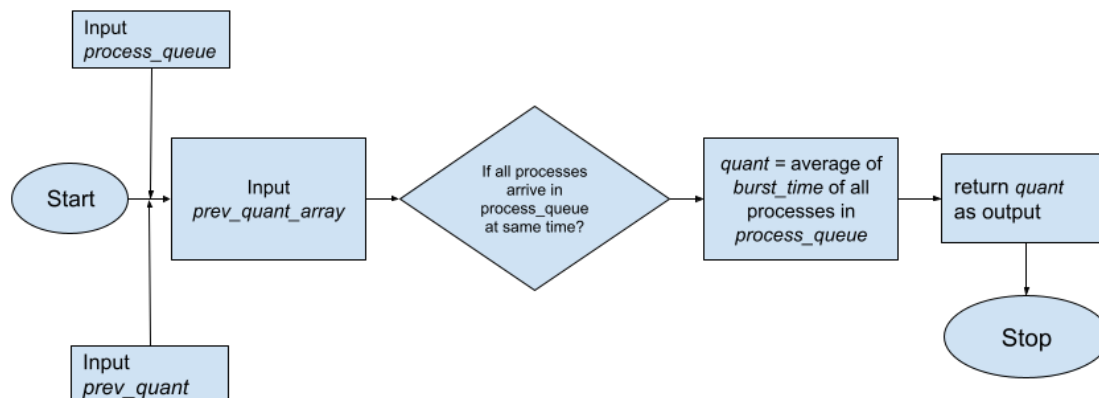
Figure 3. (a) Flowchart of quantum update: Case 1.
